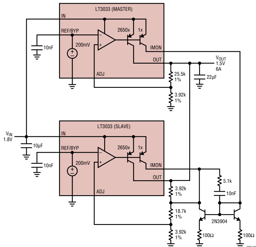
Figure 5. Paralleling Devices
