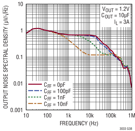
Output Noise Spectral Density C_{\text{REF/BYP}} = 10\text{nF}
