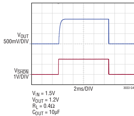
SHDN Transient Response C_{\text{REF/BYP}} = 10\text{nF}
