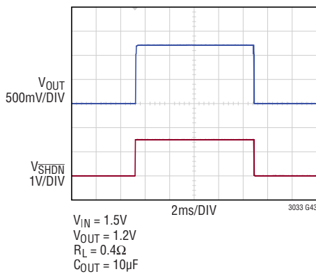
SHDN Transient Response C_{\text{REF/BYP}} = 0
