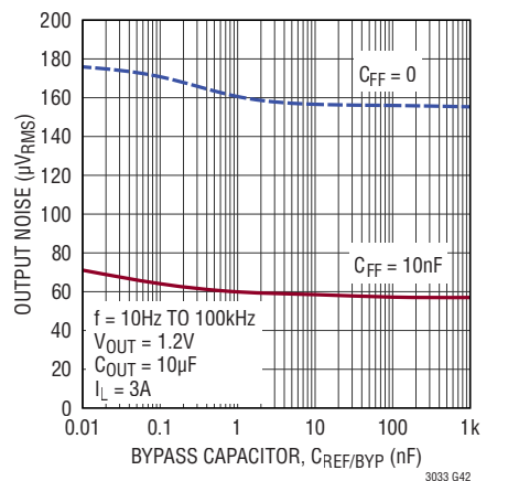
RMS Output Noise vs Bypass Capacitor ( C_{\text{REF/BYP}} )
