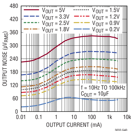
RMS Output Noise C_{\text{REF/BYP}} = 10\text{nF}, C_{\text{FF}} = 0
