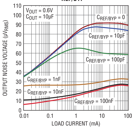
RMS Output Noise vs Load Current vs C_{REF/BYP}
