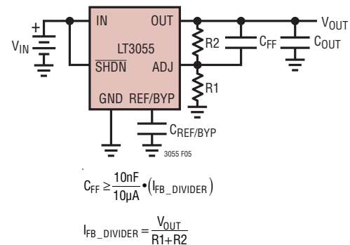
Figure 5. Feedforward Capacitor for Fast Transient Response
