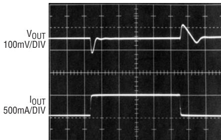
5V Transient Response C_{FF} = 10\text{nF} , I_{OUT} = 50\text{mA} to 500\text{mA}
