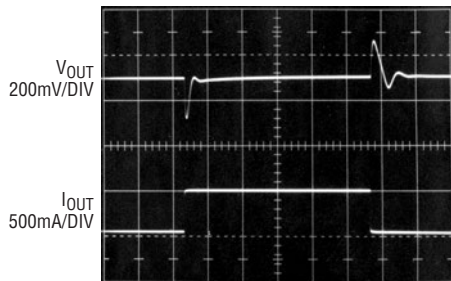
5V Transient Response C_{FF} = 0 , I_{OUT} = 50\text{mA} to 500\text{mA}
