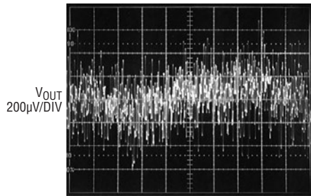
10Hz to 100kHz Output Noise C_{REF/BYP} = 10\text{nF} , C_{FF} = 0
