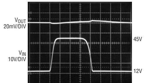
Transient Response (Load Dump)
