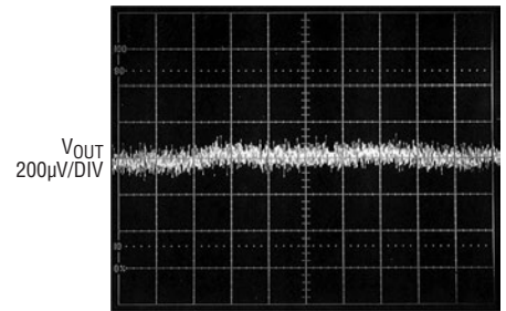
10Hz to 100kHz Output Noise C_{REF/BYP} = 10\text{nF} , C_{FF} = 10\text{nF}
