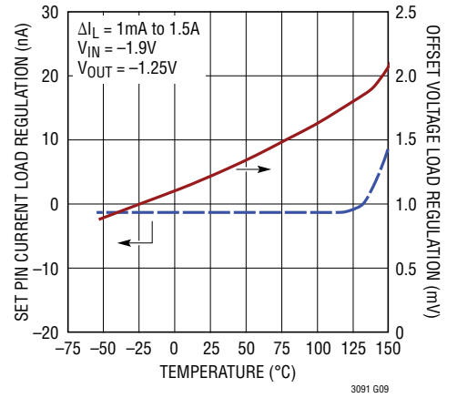
Load Regulation
