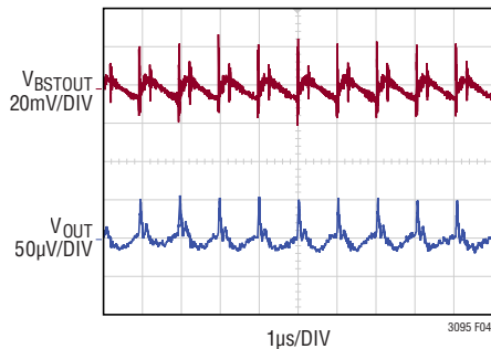
Figure 4. Output Transient Showing Spikes
