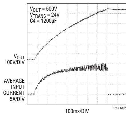
Charging Waveform
