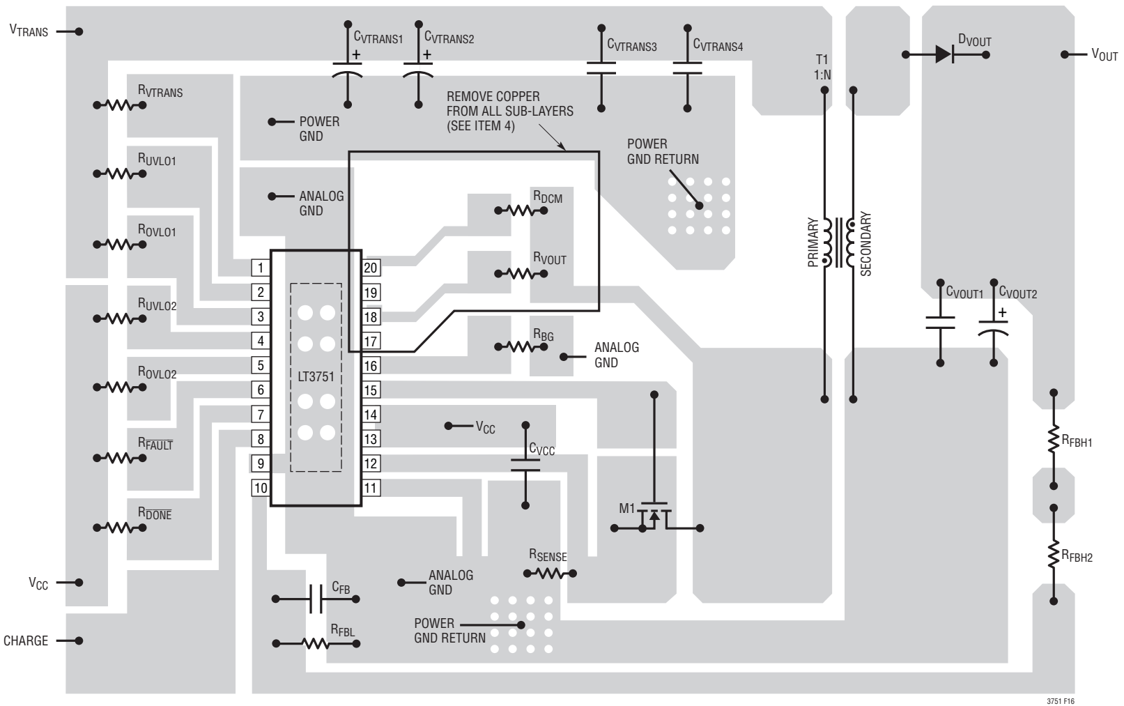
Figure 15. TSSOP Package Recommended Board Layout (Not to Scale)
