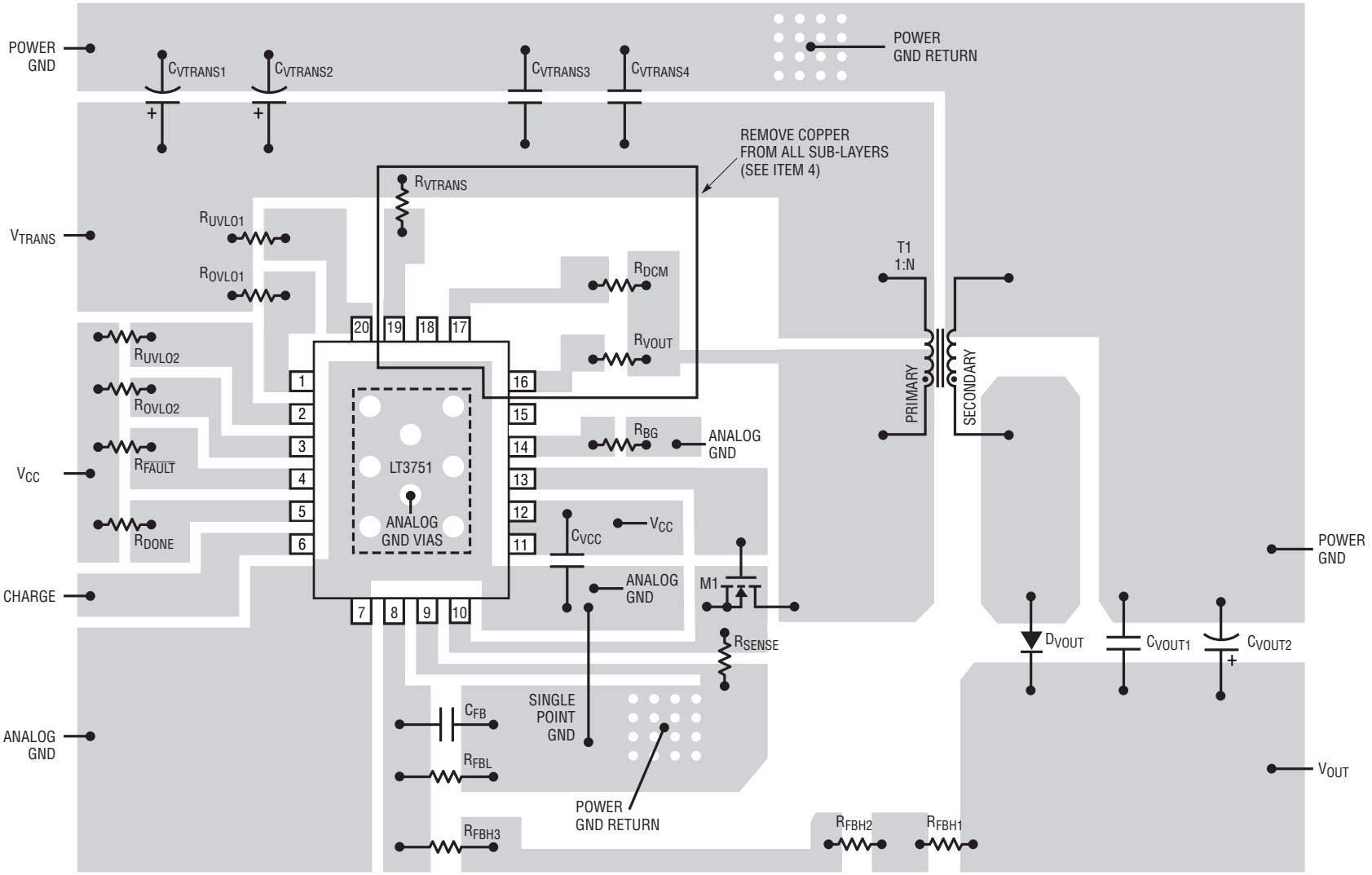
Figure 14. QFN Package Recommended Board Layout (Not to Scale)
