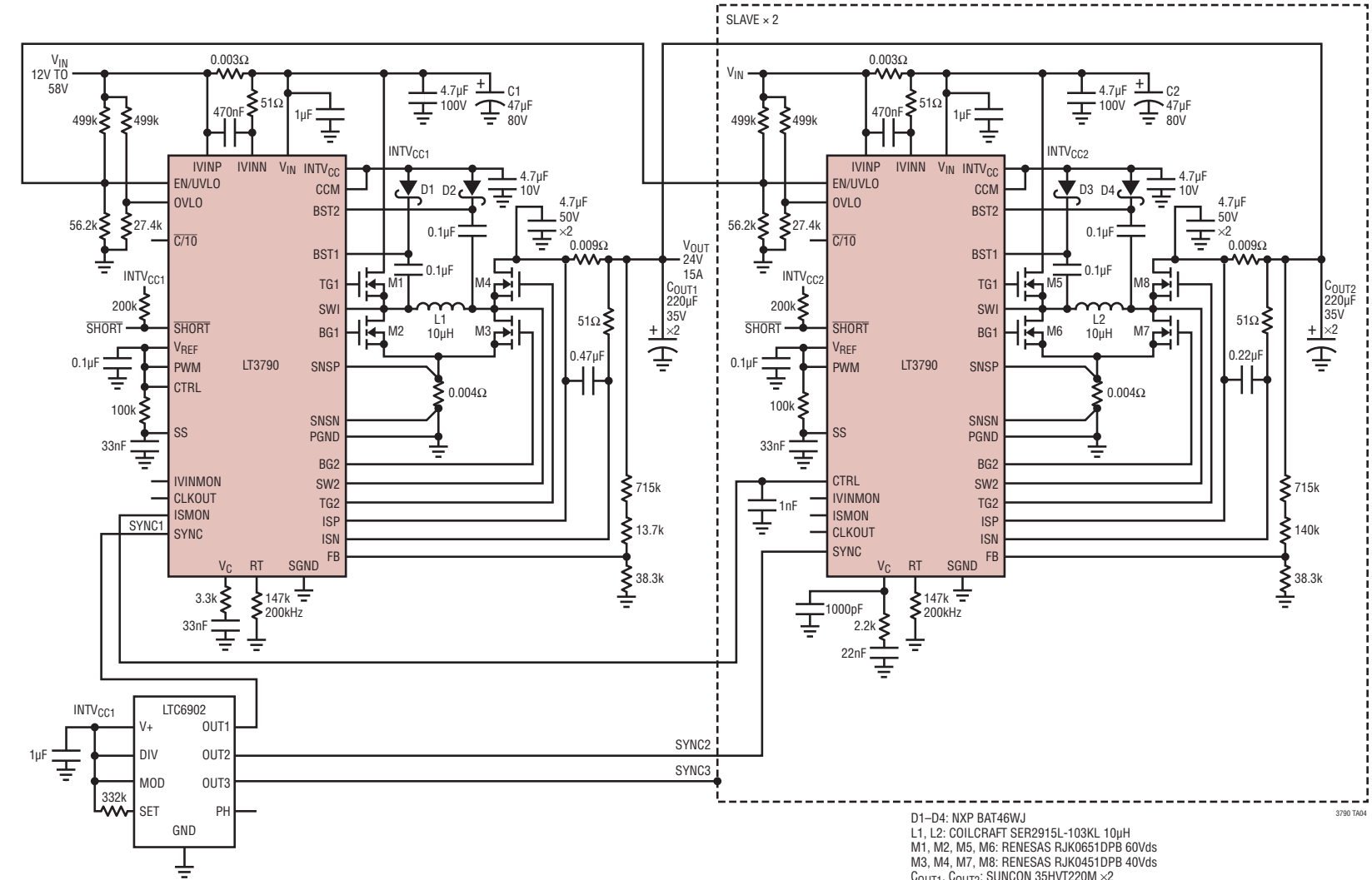
98% Efficient 360W (24V 15A) Parallel Voltage Regulators
