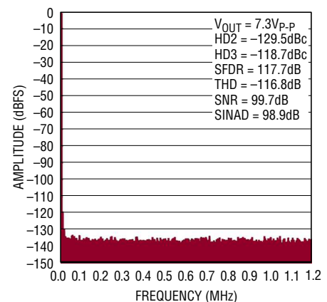
LT6237 Driving LTC2389-18 f_{\text{IN}} = 2\text{kHz} , -1dBFS, 32768-Point FFT
