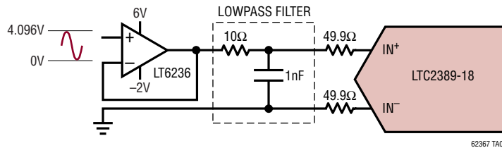
Driving a Single-Ended ADC
