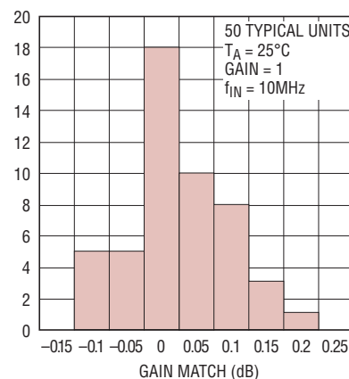
Channel to Channel Gain Matching, V_S = 5V
