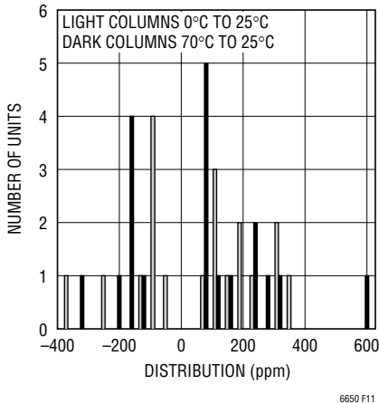
Figure 11. Worst-Case 0°C to 70°C Hysteresis
