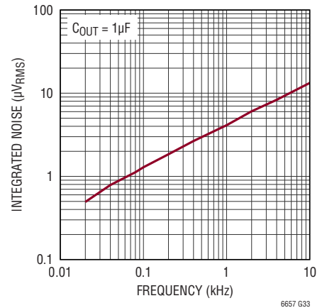
5V Integrated Noise 10Hz to 10kHz
