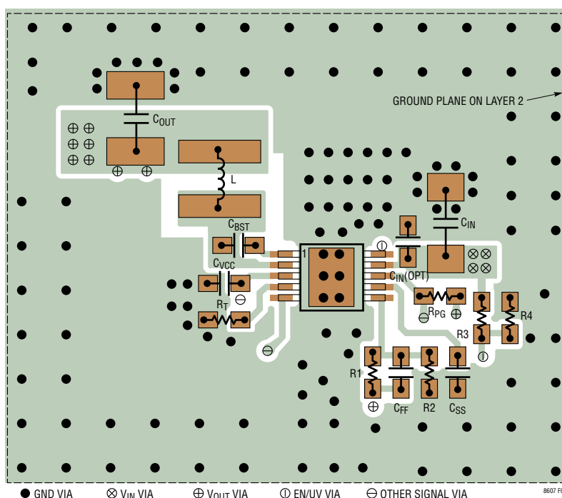
Figure 5. PCB Layout
