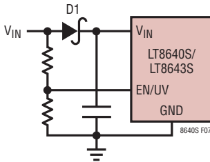
Figure 7. Reverse V_{IN} Protection
