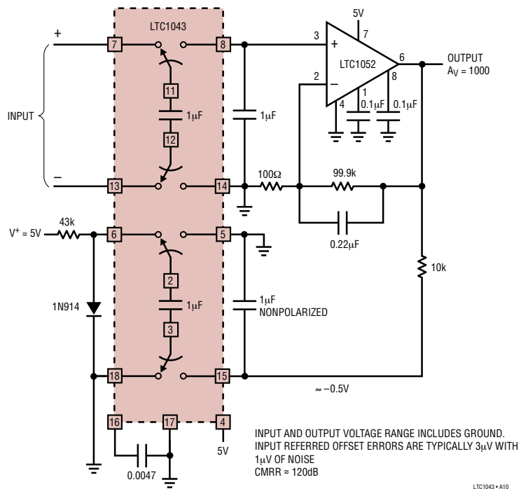
Single 5V Supply, Ultra Precision Instrumentation Amplifier
