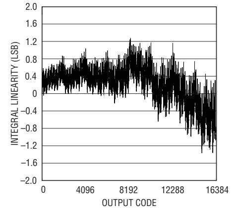
Integral Linearity End Point Fit for CH0 with Internal 2.5V Reference
