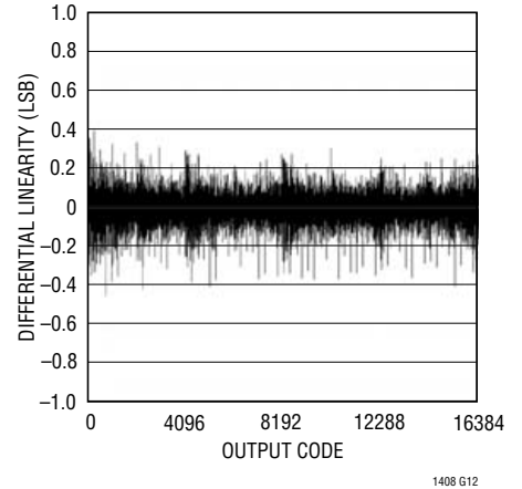
Differential Linearity for CH0 with Internal 2.5V Reference, Unipolar Mode
