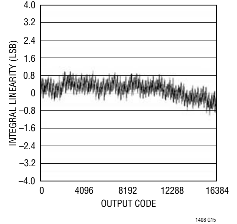
Integral Linearity End Point Fit
