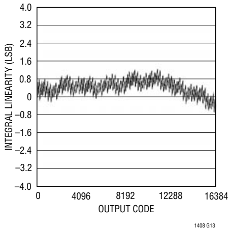
Integral Linearity End Point Fit for CH0 with Internal 2.5V Reference, Unipolar Mode
