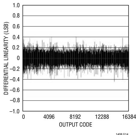
Differential Linearity for CH0 with Internal 2.5V Reference, Differential Input in Bipolar Mode
