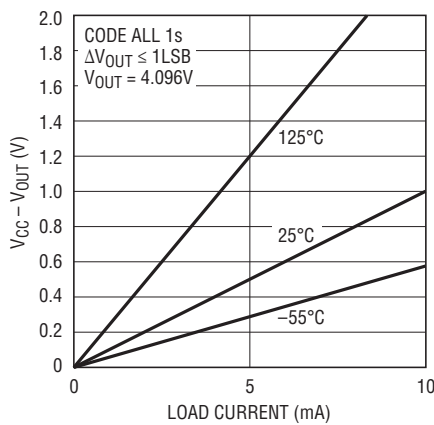
LTC1657 Minimum Supply Headroom for Full Output Swing vs Load Current
