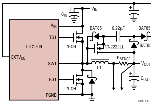
Figure 5b. Capacitive Charge Pump for EXT V CC
