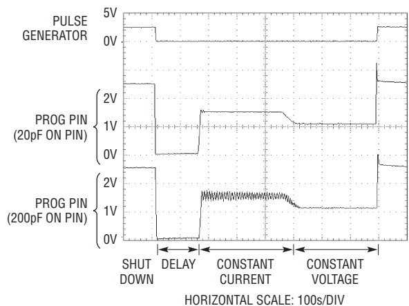
Figure 5. Stability Waveforms
