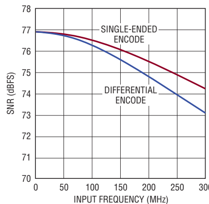
LTC2181: SNR vs Input Frequency, -1dBFS, 40Mps, 2V Range
