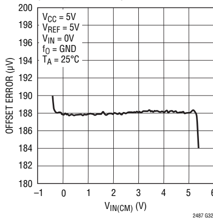
Offset Error vs V_{IN(CM)} (2x Speed Mode)
