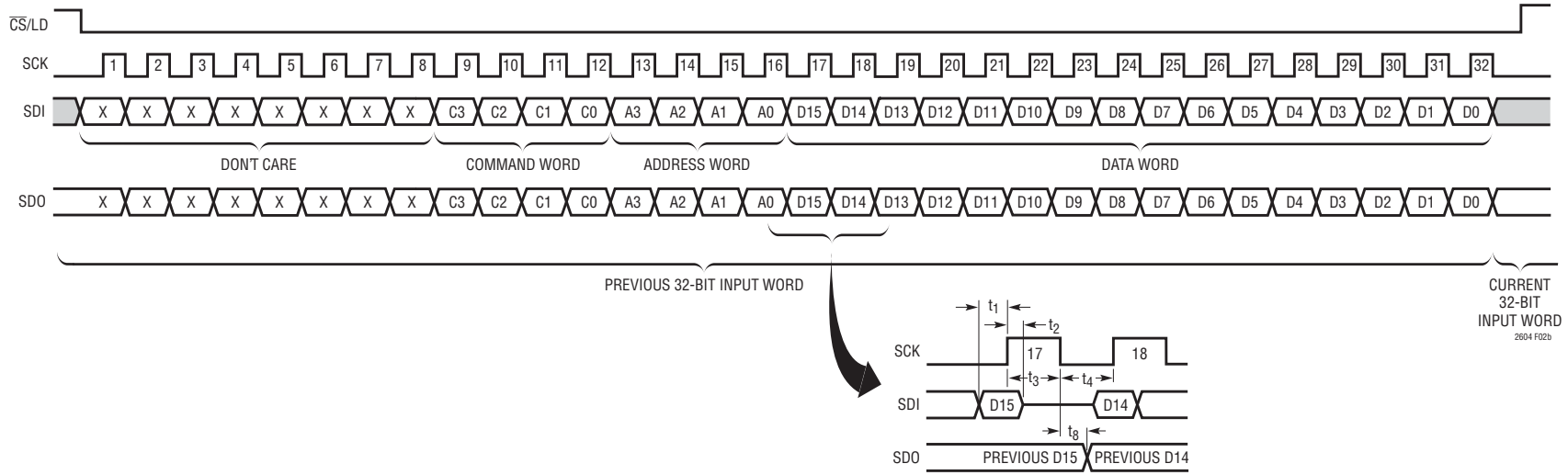
Figure 2b. LTC2604 32-Bit Load Sequence LTC2614 SDI/SDO Data Word: 14-Bit Input Code + 2 Don't Care Bits LTC2624 SDI/SDO Data Word: 12-Bit Input Code + 4 Don't Care Bits
