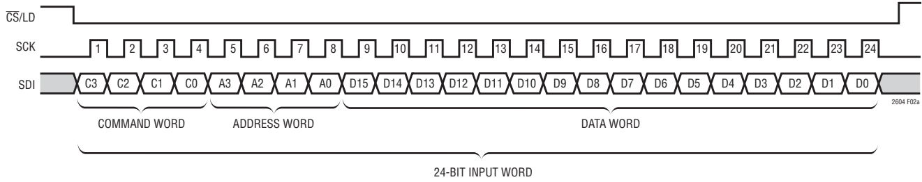
Figure 2a. LTC2604 24-Bit Load Sequence (Minimum Input Word) LTC2614 SDI Data Word: 14-Bit Input Code + 2 Don't Care Bits LTC2624 SDI Data Word: 12-Bit Input Code + 4 Don't Care Bits
