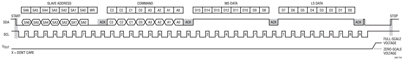
Figure 4. Typical LTC2607 Input Waveform—Programming DAC Output for Full Scale
