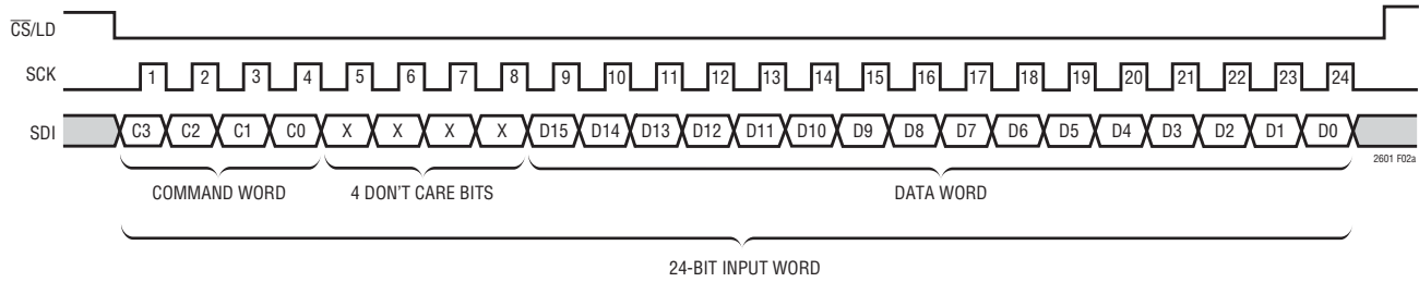
Figure 2a. LTC2601 24-Bit Load Sequence (Minimum Input Word). LTC2611 SDI Data Word: 14-Bit Input Code + 2 Don't-Care Bits; LTC2621 SDI Data Word: 12-Bit Input Code + 4 Don't-Care Bits
