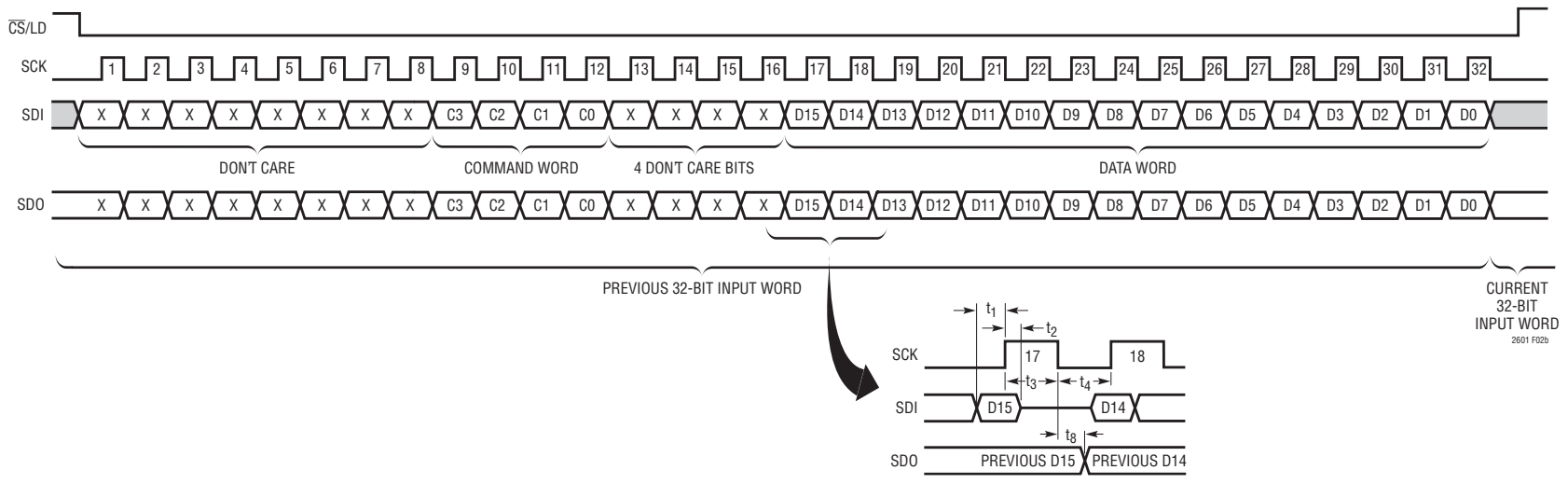
Figure 2b. LTC2601 32-Bit Load Sequence (Required for Daisy-Chain Operation). LTC2611 SDI/SDO Data Word: 14-Bit Input Code + 2 Don't-Care Bits; LTC2621 SDI/SDO Data Word: 12-Bit Input Code + 4 Don't-Care Bits
