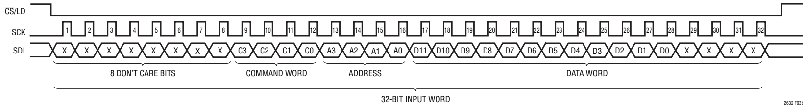
Figure 3b. LTC2632-12 32-Bit Load Sequence LTC2632-10 SDI Data Word: 10-Bit Input Code + 6 Don't-Care Bits; LTC2632-8 SDI Data Word: 8-Bit Input Code + 8 Don't-Care Bits
