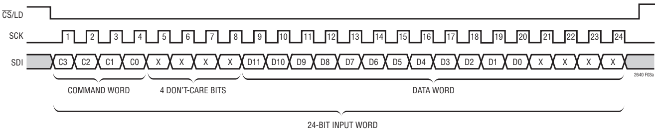
Figure 3a. LTC2640-12 24-Bit Load Sequence (Minimum Input Word). LTC2640-10 SDI Data Word: 10-Bit Input Code + 6 Don't-Cares Bits; LTC2640-8 SDI Data Word: 8-Bit Input Code + 8 Don't-Cares Bits
