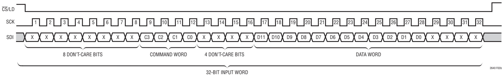
Figure 3b. LTC2640-12 32-Bit Load Sequence LTC2640-10 SDI Data Word: 10-Bit Input Code + 6 Don't-Cares Bits; LTC2640-8 SDI Data Word: 8-Bit Input Code + 8 Don't-Cares Bits
