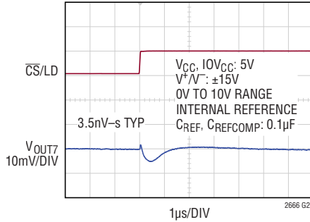
DAC-to-DAC Crosstalk
