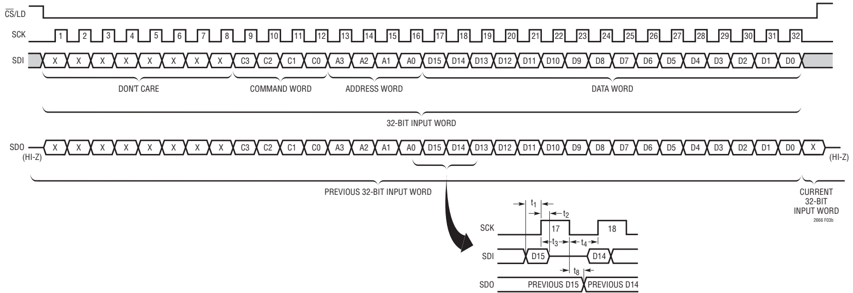
3b. LTC2666-16 32-Bit Load Sequence. LTC2666-12 SDI/SDO Data Word Is 12-Bit Input Code + 4 Don't-Care Bits
