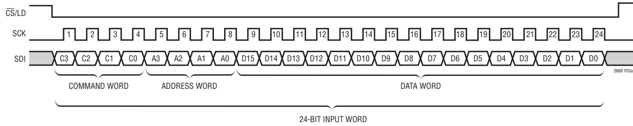
3a. LTC2668-16 24-Bit Load Sequence (Minimum Input Word). LTC2668-12 SDI Data Word Is 12-Bit Input Code + 4 Don't-Care Bits
