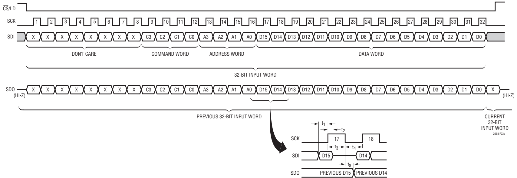
3b. LTC2668-16 32-Bit Load Sequence. LTC2668-12 SDI/SDO Data Word Is 12-Bit Input Code + 4 Don't-Care Bits
