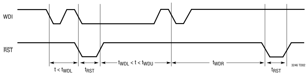
Watchdog Timing
