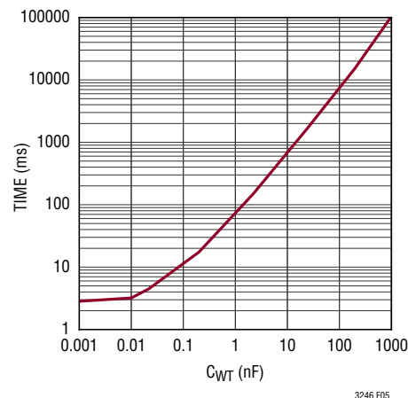
Figure 5. External Watchdog Timeout Period vs C_{\text{WT}} Capacitance
