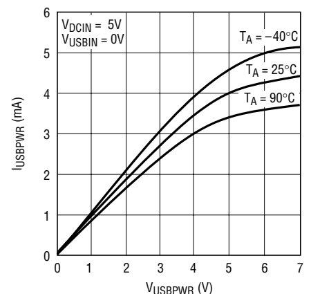
IUSBPWR Pin I-V Curve
