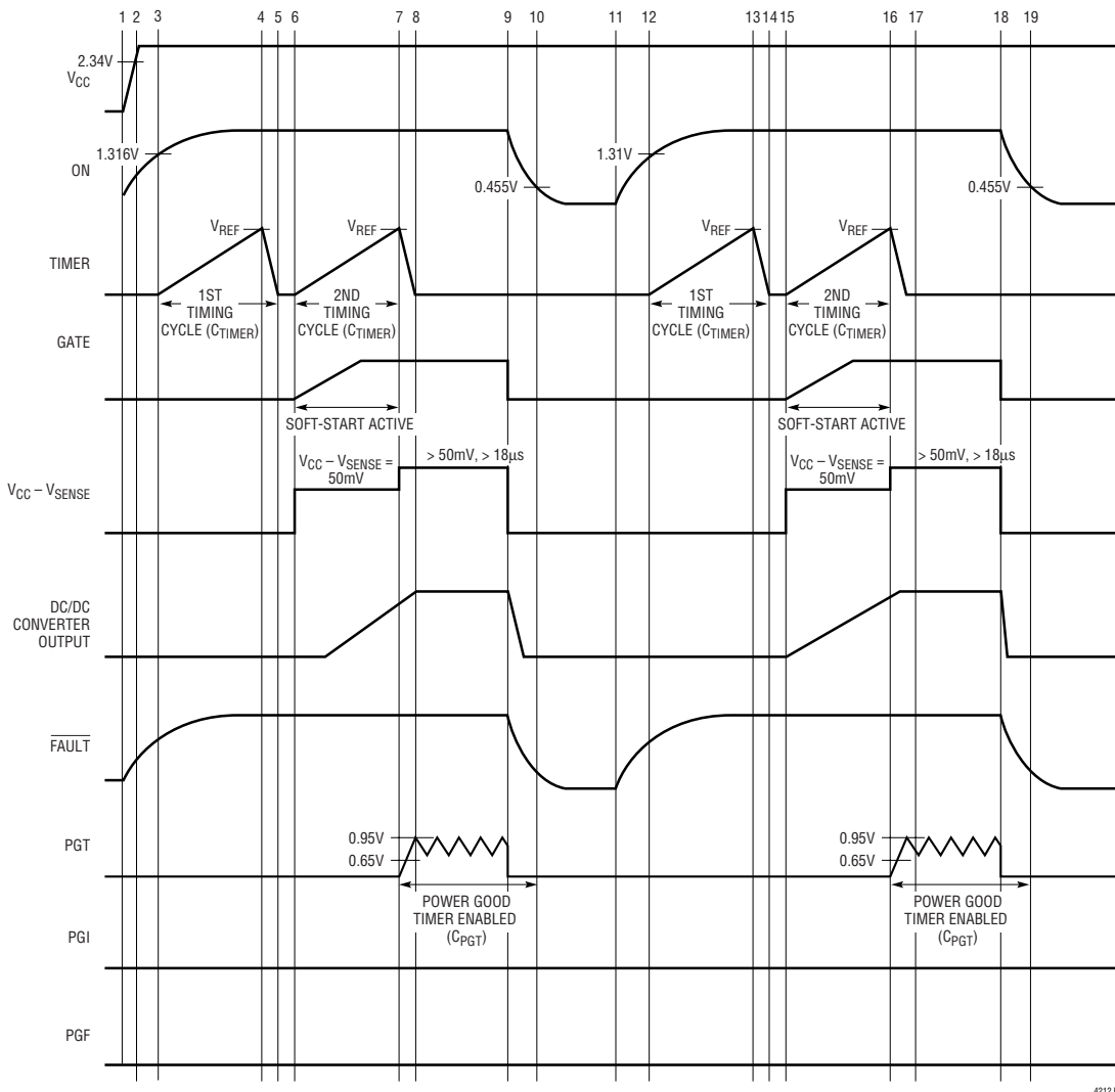
Figure 6. Autoretry Sequence
