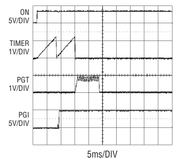
Power-Up Waveforms
