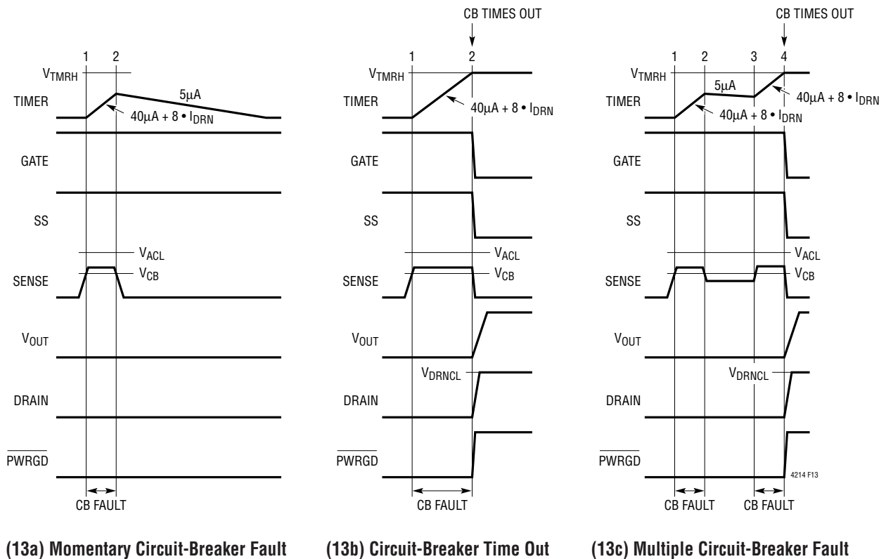
Figure 13. Circuit-Breaker Timing Behavior (All Waveforms are Referenced to V_{\text{EE}} )
