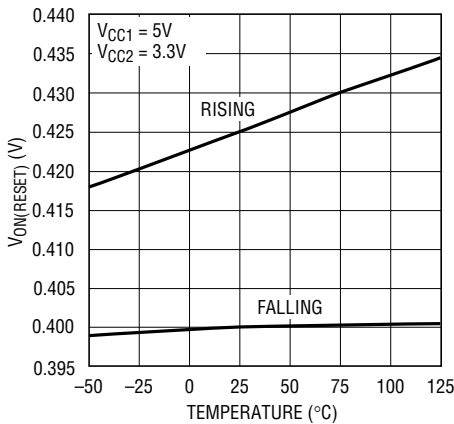
V_{ON(RESET)} vs Temperature
