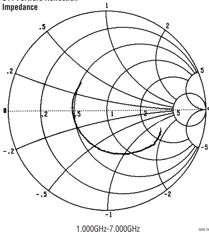
S11 Forward Reflection Impedance
