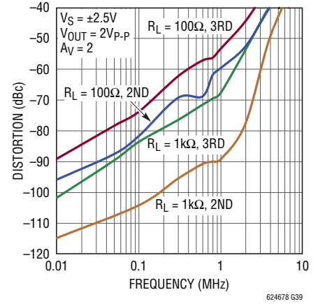
Distortion vs Frequency ( A_V = 2, 5V )
