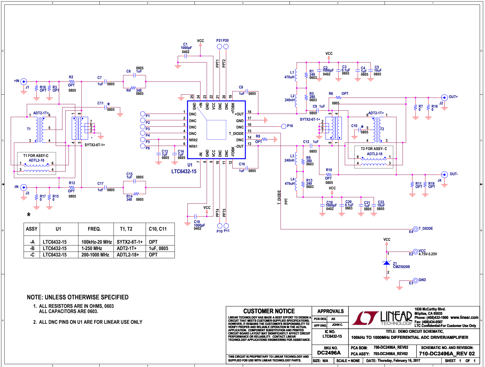
Figure 2. DC2496A Balanced Amplifier Circuit – 50Ω Input and 50Ω Output
