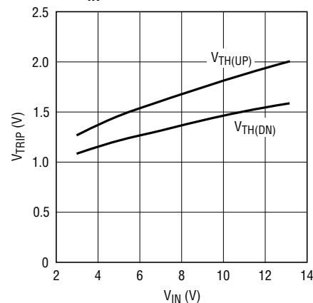
\overline{\text{SHDN}} Input Voltage Thresholds vs V_{IN}
