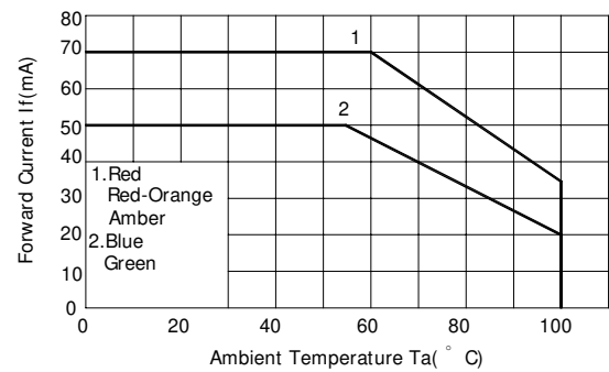
Fig.4 Forward Current vs. Ambient Temperature ( R_{\theta j-a}=300^{\circ}\text{C/W} )
