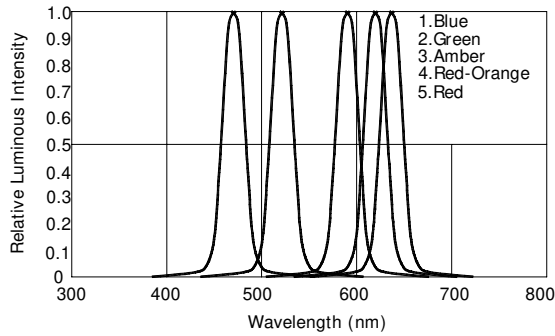
Fig.1 Relative Luminous Intensity vs. Wavelength
