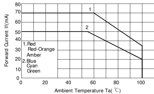
Fig.4 Forward Current vs. Ambient Temperature ( \theta_{j-a}=300\text{ }^{\circ}\text{C/W} )
