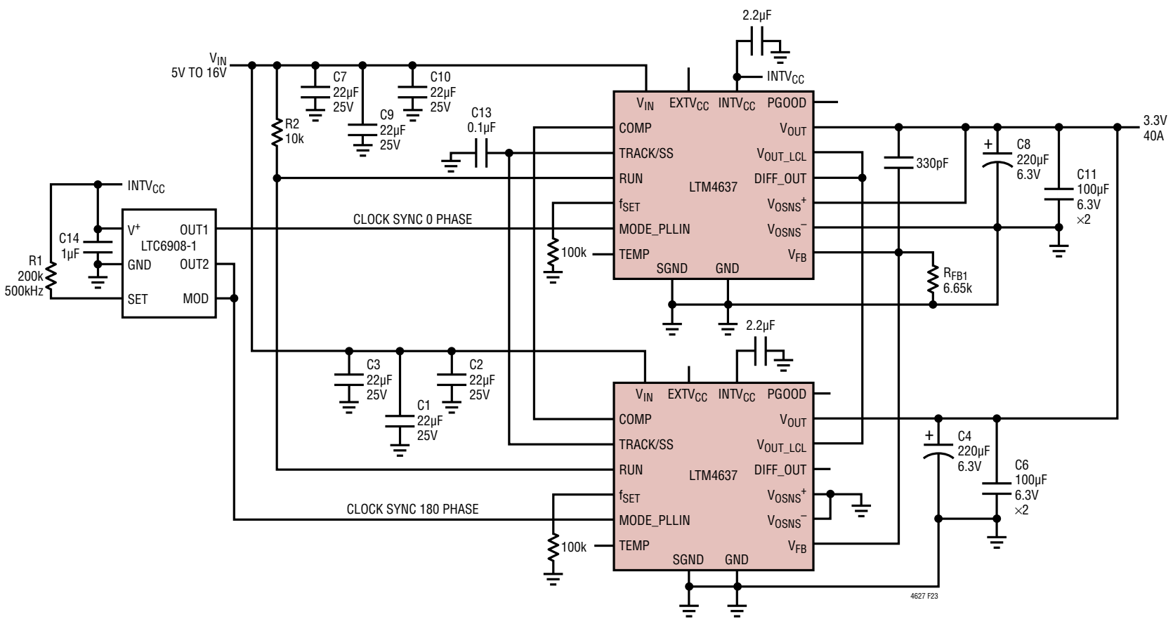
Figure 23. 3.3V at 40A, Two Parallel Outputs with 2-Phase Operation
