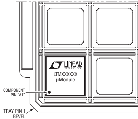
PACKAGE IN TRAY LOADING ORIENTATION
