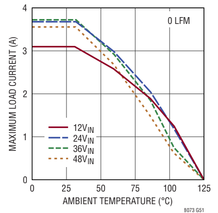
Derating, V_{OUT} = -5\text{V} , BIAS = 0V, DC2389A Demo Board
