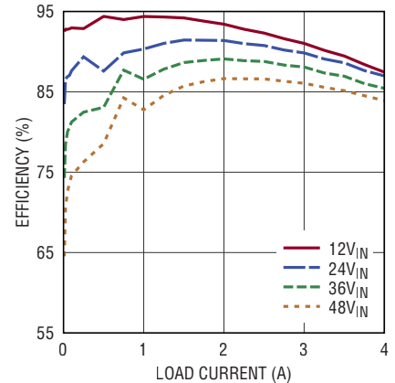
Efficiency, V_{OUT} = 5\text{V} , BIAS = 5V
