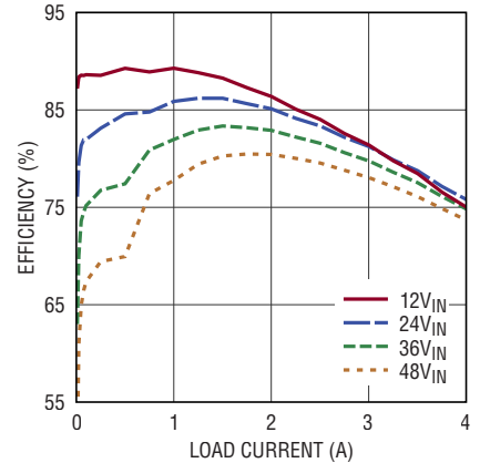
Efficiency, V_{OUT} = 2\text{V} , BIAS = 5V
