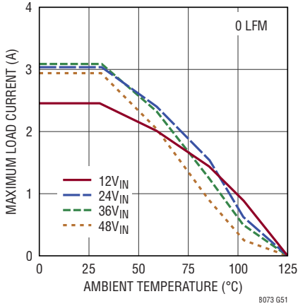
Derating, I-Grade V_{OUT} = -8\text{V} , BIAS = 0V, DC2389A Demo Board
