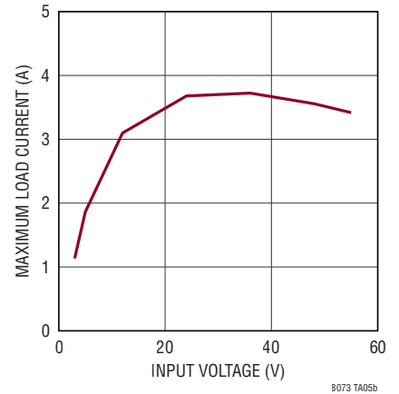
Maximum Load Current vs V IN , BIAS = 0V
