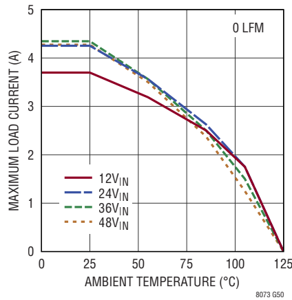
Derating, V_{OUT} = -3.3\text{V} , BIAS = 0V, DC2389A Demo Board
