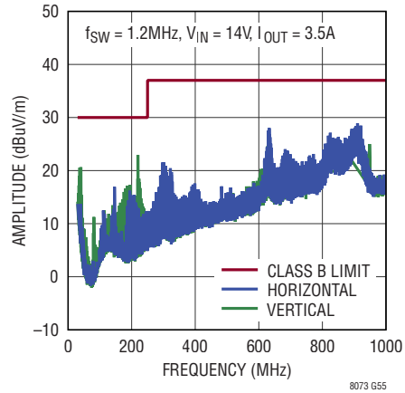
CISPR22 Class B Radiated DC2389A Demo Board, V_{OUT} = 5\text{V} No Filter (FB1 Short, C8, C9 Open)
