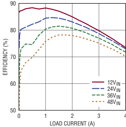
Efficiency, V_{OUT} = 1.5\text{V} , BIAS = 5V
