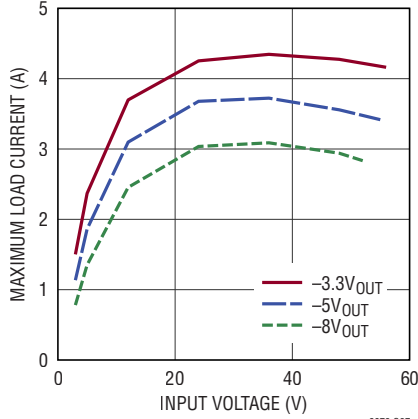
Maximum Load Current vs V_{IN} BIAS = 0V
