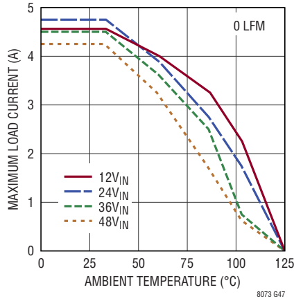
Derating, V_{OUT} = 8\text{V} , BIAS = 5V, DC2389A Demo Board
