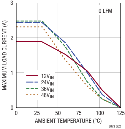
Derating, I-Grade V_{OUT} = -12\text{V} , BIAS = 0V, DC2389A Demo Board
