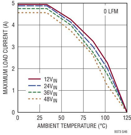
Derating, V_{OUT} = 5\text{V} , BIAS = 5V, DC2389A Demo Board
