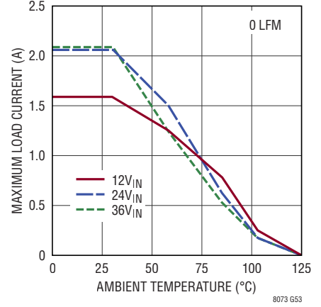
Derating, I-Grade V_{OUT} = -15\text{V} , BIAS = 0V, DC2389A Demo Board
