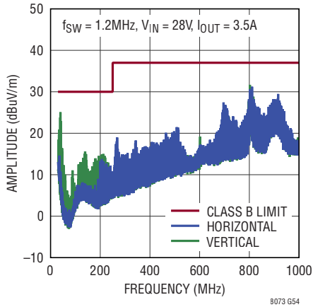
CISPR22 Class B Radiated DC2389A Demo Board, V_{OUT} = 5\text{V} No Filter (FB1 Short, C8, C9 Open)
