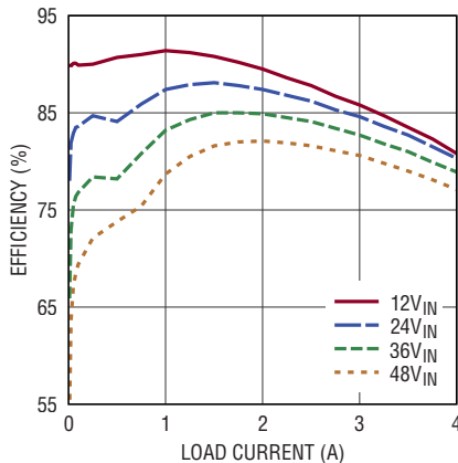
Efficiency, V_{OUT} = 2.5\text{V} , BIAS = 5V
