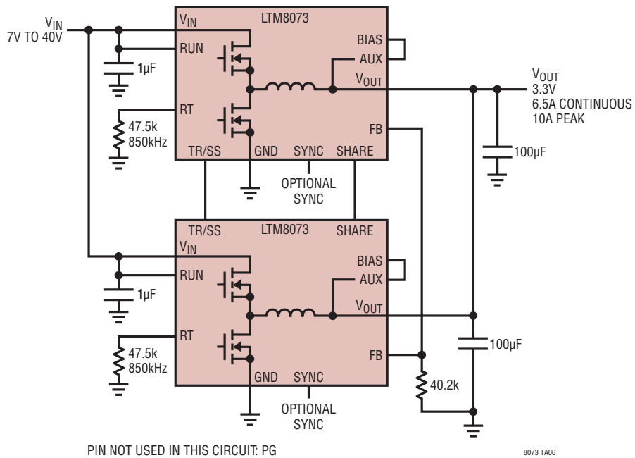
Use Two LTM8073s Powered from the Same Input Source to Get More Output Current
