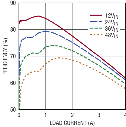
Efficiency, V_{OUT} = 0.8\text{V} , BIAS = 5V
