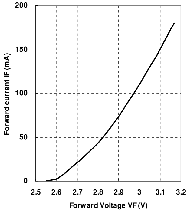
Fig 3. Forward Current
