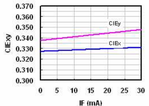
Fig.7. CIExy vs. Forward Current
