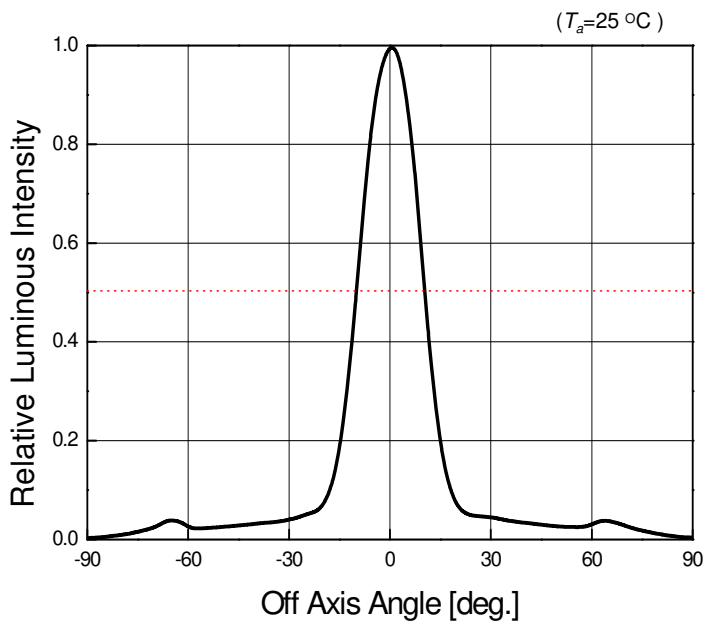
Radiation Diagram
