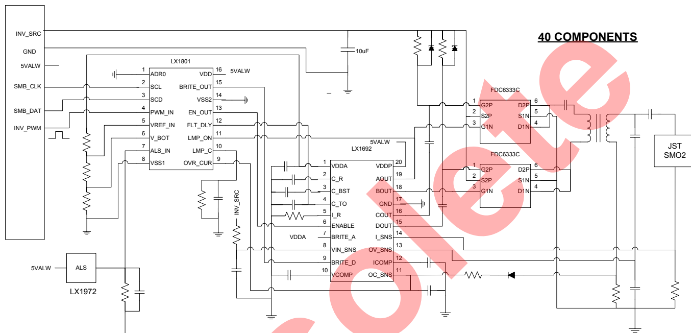
Figure 2 – Typical Application
