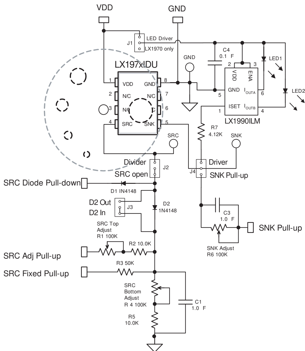
Figure 2 – Schematic
