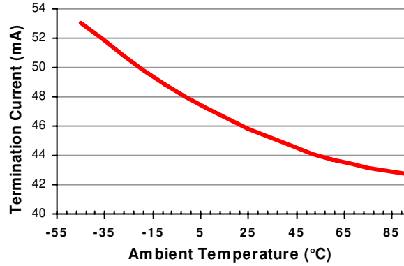
Chart 2 – Termination Current over Temperature
