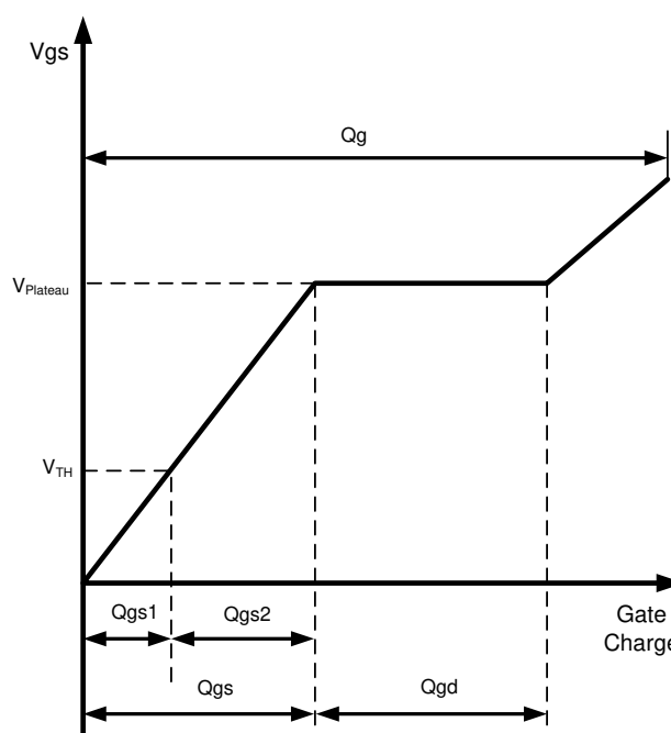
Figure 15. Gate Charge Definitions
