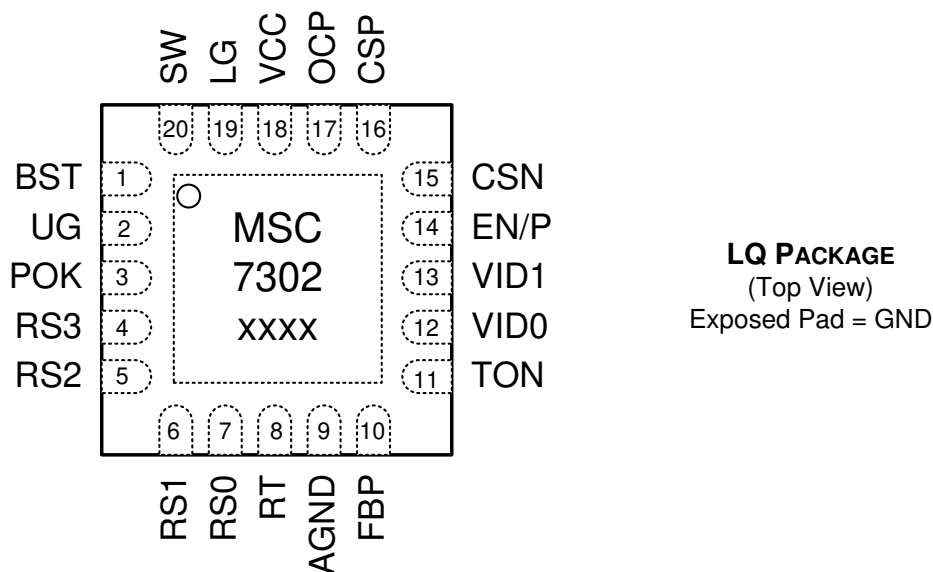
Figure 3: Pinout
