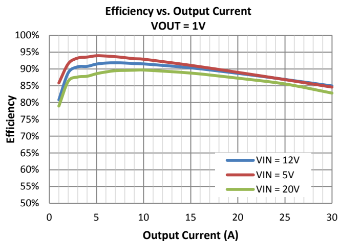
Figure 8. Efficiency
