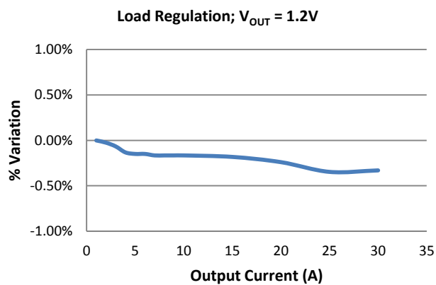
Figure 10. Load Regulation
