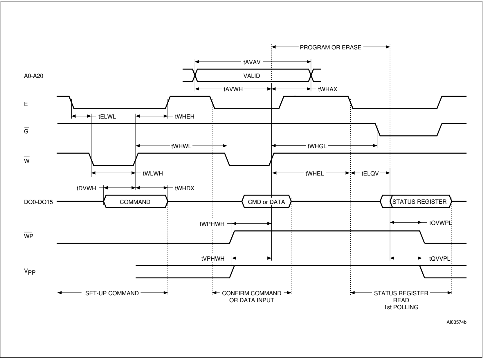
Figure 11. Write AC Waveforms, Write Enable Controlled
